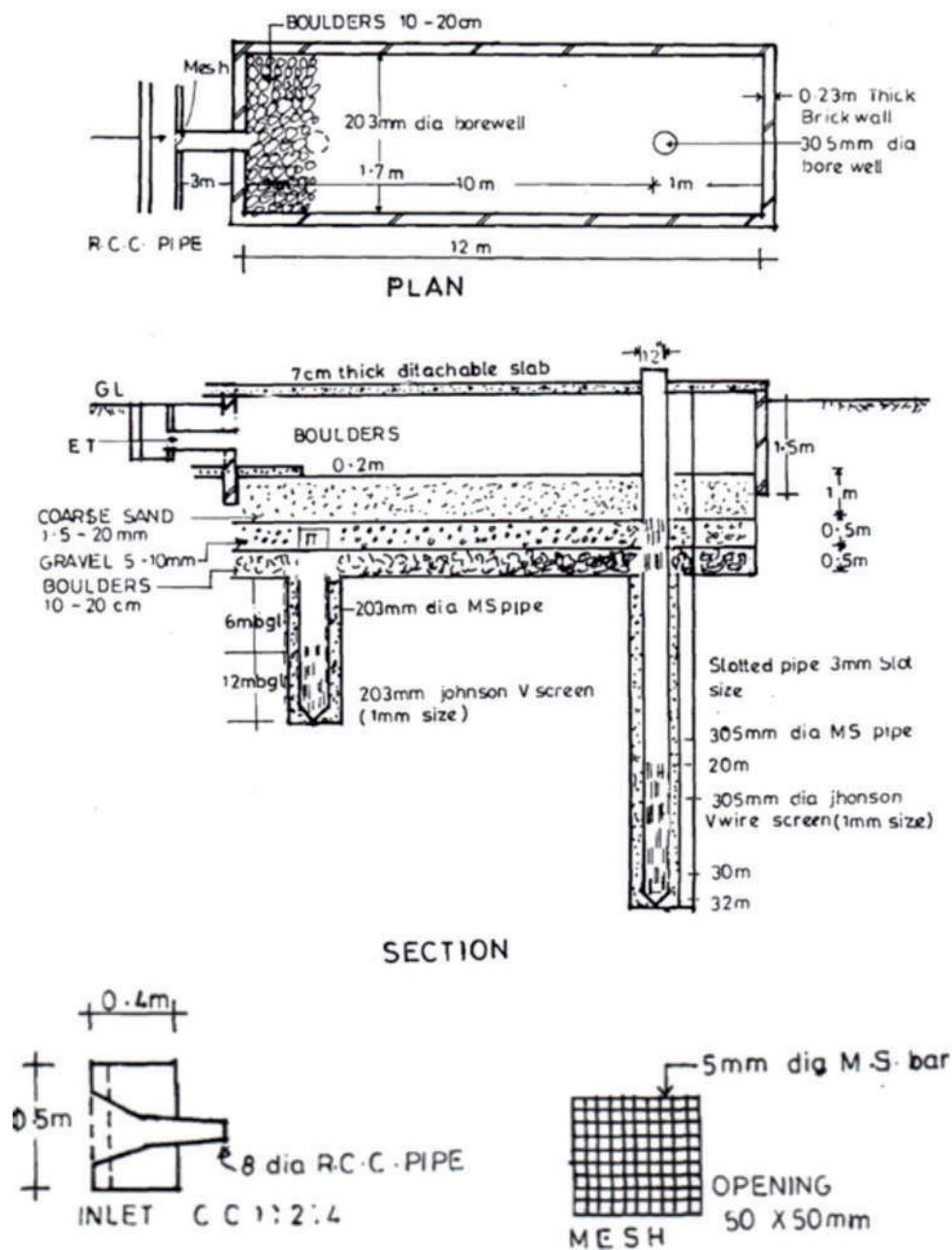
Drg. No. 23 Size of recharge trench cum recharge wells
